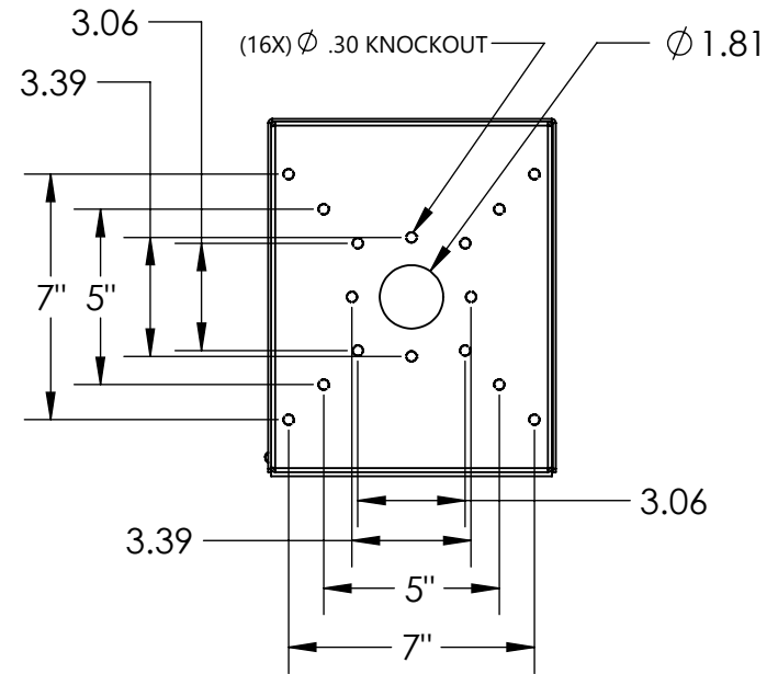
CONTROL4/2N SINGLE UNIT CUTOUT (SURFACE)
